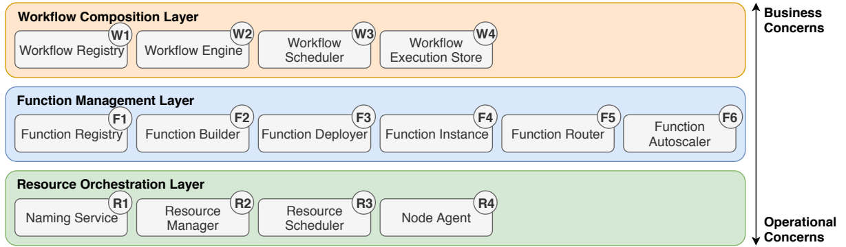
Figure 1: The SPEC-RG reference architecture for FaaS platforms (reproduced from [10]).
