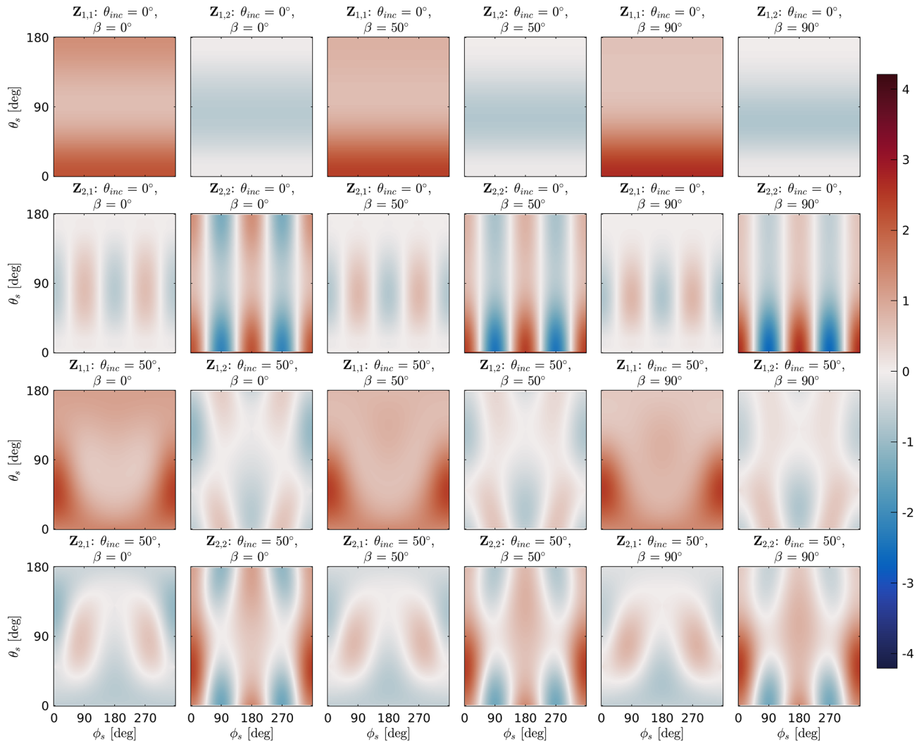
Figure 11. The upper-left block of the normalized scattering matrix \hat{\mathbf{Z}} of large plate aggregate with a volume-equivalent diameter of 427\ \mu\text{m} (Fig. 4) at 167 GHz, as a function of the polar scattering angle \theta_s and the azimuth scattering angle \phi_s for a set of tilt angles \beta and incidence angles \theta_{\text{inc}} . A volume-equivalent diameter of 427\ \mu\text{m} at 167 GHz corresponds to size parameter x \approx 0.75 .
