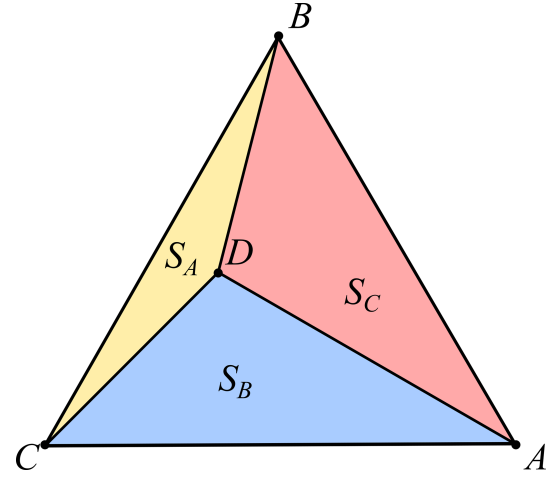
Figure C1. Geometry of triangular barycentric interpolation.
