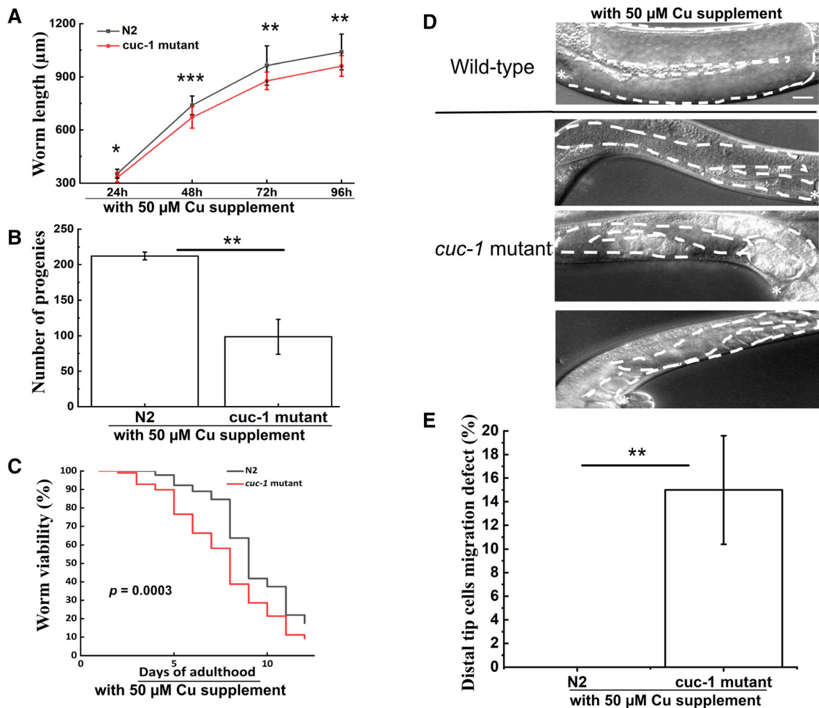
Fig. 5 Characterization of cuc-1 mutant versus wild-type (N2) C. elegans at 24, 48, 72 h incubation post L1 stage (condition with 50 \mu M supplemental Cu). a Growth assay ( n_{\text{group}}=25 ). b Brood size assay ( n_{\text{group}}=10 ). c Life span assay ( n_{\text{group}}=100 ). d Examples of DTC migration defects found in cuc-1 mutant C. elegans . Asterisks indicate vulva. White dashed lines indicate
