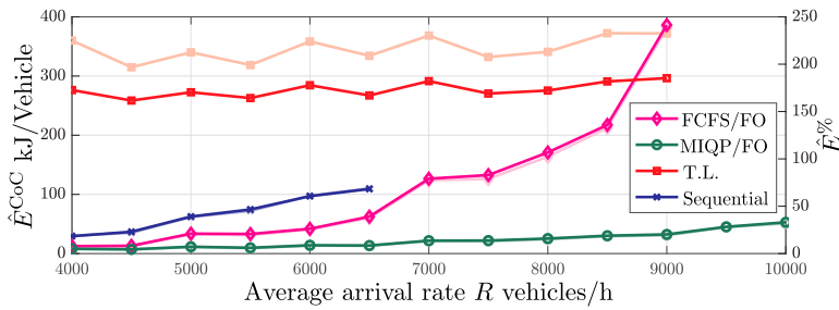
Figure 4. Energy cost of coordination: percentage increase \hat{E}^{\%} (solid line, right axis); and CoC increase \hat{E}^{\text{CoC}} (pale lines, left axis). Colour coding as in Figure 3.
