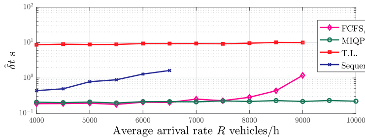
Figure 5. Travel time delay compared to the Overpass solution.
