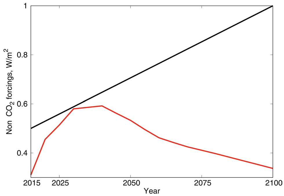
Extended Data Fig. 4 | Exogenous path for non-CO 2 forcings. The black line depicts the standard DICE 2016R2 assumption; the red line shows the updated path based on the REMIND SSP2.6 scenario.
