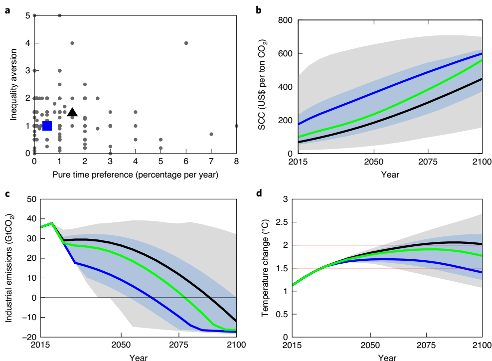
Fig. 2 | Climate policy pathways in the updated DICE model. a , Graph showing each expert's value judgements on discounting parameters (rate of pure time preference; inequality aversion; n=173 ). The black triangle (1.5%; 1.45) indicates the choice of discount parameters by Nordhaus 34 and the blue square (0.5%; 1) the median expert view on intergenerational welfare. b-d , Graphs showing the 95th (grey-shaded area) and 66th (blue-shaded area) percentile ranges in terms of intergenerational fairness for three climate policy measures: the SCC ( b , in US$ per ton), industrial emissions ( c , in GtCO 2 ) and global mean temperature increases from 1850 to 1900 levels ( d , in °C). These ranges do not correspond to confidence intervals relating to uncertainty about forecasts, rather they capture how the disagreement about discounting parameters affects the optimal paths when incorporated into our updated DICE model. Panels b-d also compare climate policy pathways implied by Nordhaus' discounting in this updated DICE (black line) to those resulting from the median expert view (blue line) and the median expert path (green line). While Nordhaus' discounting implies an optimal carbon price of US$82 in 2020, in our updated DICE the median expert path (or view) translates into a value of US$119 (or US$208) in 2020.
