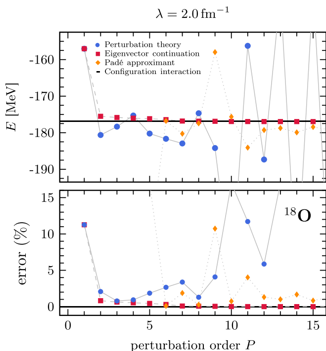
FIG. 2. Ground-state energy of {}^{18}\text{O} for BMBPT (blue circles), BMBPT-based EC (red squares), and BMBPT-based Padé (yellow diamonds) as a function of the perturbative order P against exact CI diagonalization (full line) for \lambda = 2.0 \text{ fm}^{-1} . Top panel: absolute energies. Bottom panel: relative error to the CI result.
