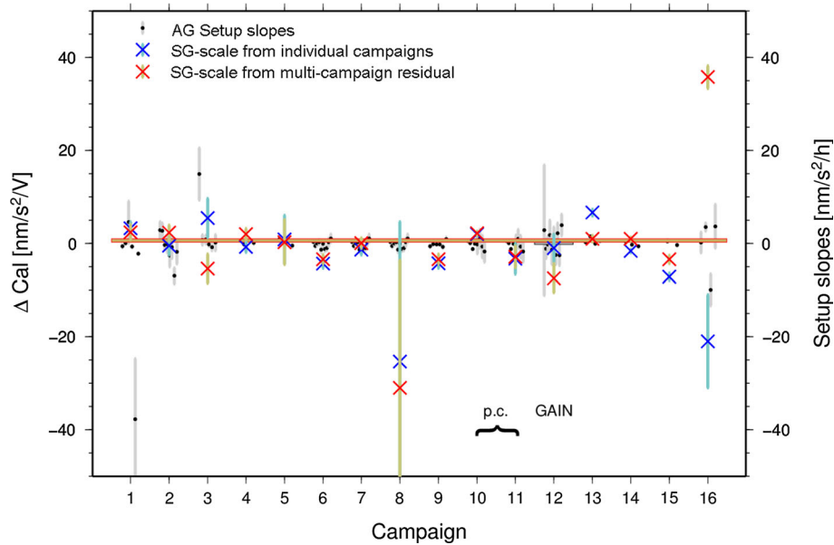
Fig. 2 AG setup slopes and SG scale factor. The multi-campaign's solution for the scale factor is shown as the yellow horizontal line outlined by a red box to show its uncertainty. The value determined from the GAIN campaign in parallel with campaign no. 12 (201502b) is shown as a short horizontal grey bar (zero line), its thickness representing the uncertainty; all other scale factor ordinates represent differences to GAIN. Residual, campaign-related signatures are determined from covariation with the multi-campaign residual evaluated within the cam-
