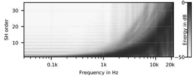
Fig. 1. Normalized logarithmic energy distribution of the head-related transfer functions (HRTFs) of the employed Neumann KU100 dummy head over frequency and SH order n . The color encodes the energy ranging from -50 dB normalized to the maximum values for each frequency bin.
