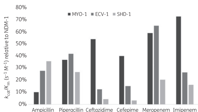
Figure 2. Relative catalytic efficiencies [ k_{cat}/K_m ( s^{-1}M^{-1} )] of MYO-1, ECV-1 and SHD-1 compared with NDM-1.
