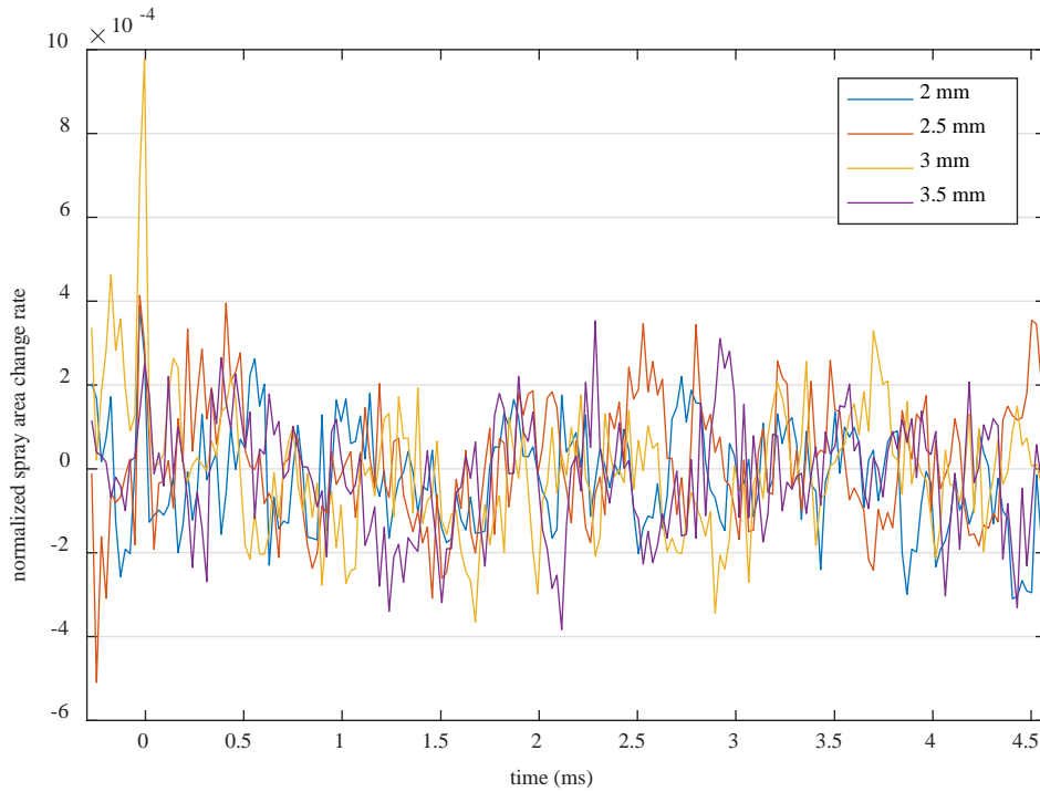
Figure 5 Normalized spray area change rate for various d when the injection pressure was 5 bar.
