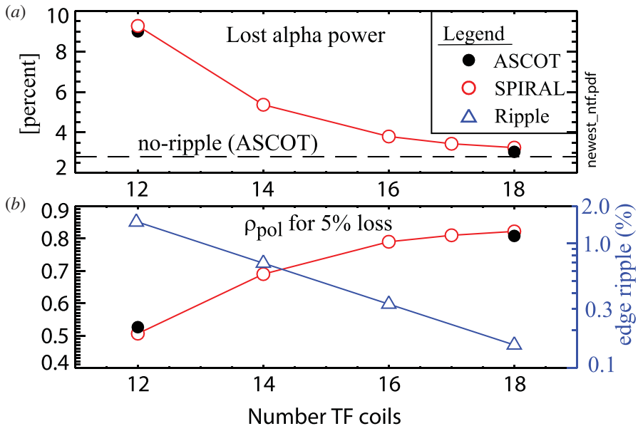
FIGURE 8. (a) Computed percentage of lost-alpha power for the SPARC V1E coil shape as a function of number of TF coils. (b) The value of birth \rho_{\text{pol}} at which the volume-integrated alpha power losses (from \rho_{\text{pol}}=0 ) equal 5% of the total alpha power losses.
