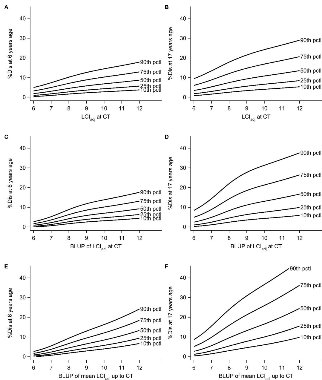
Figure E2. Estimated percentiles of total airway disease (%Dis) at six and 17 years of age vs LCI_{adj} at CT (+/- 3 days) (A, B), BLUP of LCI_{adj} at CT (C, D), and BLUP of mean LCI_{adj} up to CT (E, F). The BLUP is the best linear unbiased prediction using all available MBW data up and including the time-point of CT. Percentile curves were derived from mixed effects models on logit-transformed outcomes, using all available longitudinal MBW and CT data.
