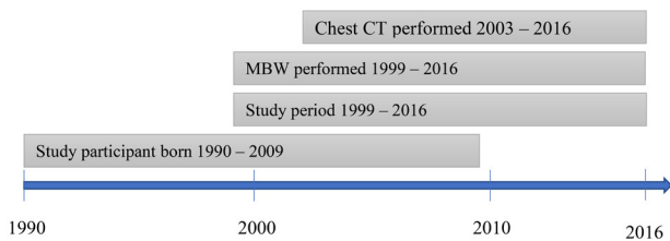
Figure 1 Longitudinal overview of the cohort and the main outcomes of the study. Multiple breath washout (MBW) was performed annually between 1999–2012 and every 6 months between 2013 and 2016. Chest CT was performed from the age of 6 years and repeated every third year.
