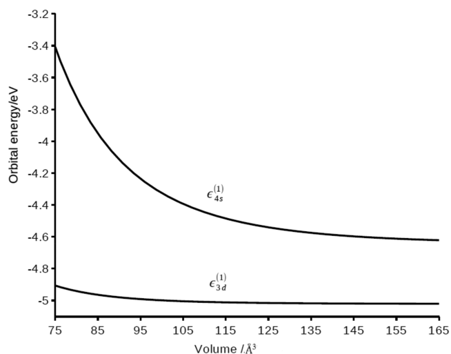
Figure 2. Compressed scandium atom: first-order orbital energies (eV) \epsilon_{nl}^{(1)} of the 4s and 3d orbitals as a function of the compression volume (Å 3 ).
