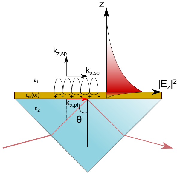
Figure 3.1: Surface plasmon excitation using the Kretschmann-Raether configuration.
