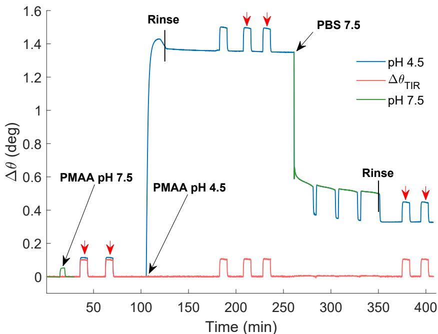
Figure 4.2: SPR measurements during injection of PMAA to saturation on top of a 20 kDa PEG brush at pH 4.5 and 7.5. The blue trail corresponds to \Delta\theta_{SPR} at pH 4.5 and green trails to \Delta\theta_{SPR} at pH 7.5. The red trail corresponds to bulk liquid changes via the \Delta\theta_{TIR} . Red arrows mark examples of selected height-probing injections with Dextran (10 mg/ml, 100 kDa, pH 4.5). Black arrows mark the starting points upon injecting PMAA (100 \mu g/ml, 8 kDa, pH 4.5) and PBS solution at 7.5. "Rinse" mark returning to pH 4.5 solution.
