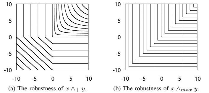
Fig. 8: Isobar plots of the robustness of the two semantics of \wedge . Here, negative robustnesses represent false VBBools.
