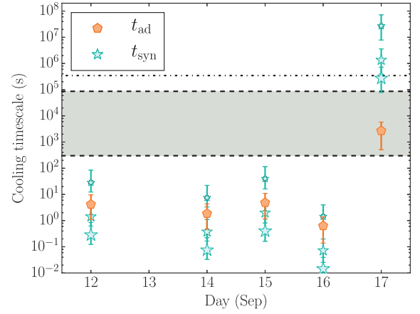
Figure 5. Adiabatic and radiative cooling time-scales of the compact jet emission from our September 12–17 epochs. Orange pentagons indicate the adiabatic time-scale during each epoch; cyan stars indicate the radiative time-scale for electrons with Lorentz factors of 100, 20, and 1. Larger stars indicate larger electron Lorentz factors. The grey band represents the compact jet \nu_{\text{break}} variability time-scales; the bottom dashed line corresponds to the interobservation variability time-scale of a few minutes and the top dashed line corresponds to the time between the September 16 and 17 observations. The dot-dashed line corresponds to the time between the September 17 and 21 observations, which is the most conservative estimate for the rate at which the compact jet was quenched. The variation of \nu_{\text{break}} inferred from our observations implies that the acceleration region of the jet is moving away from the BH system on adiabatic/dynamical time-scales.
