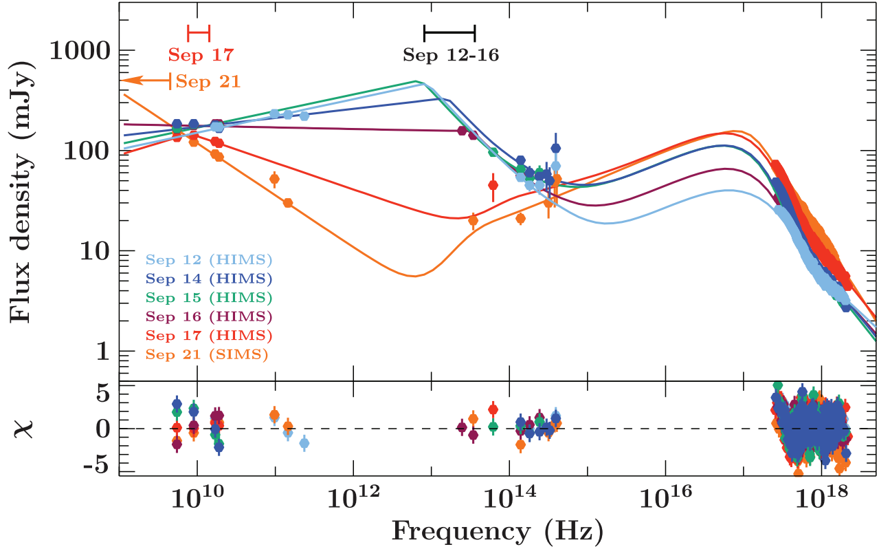
Figure 1. Broad-band multiwavelength modelling of MAXI J1535–571 during the rise phase of its 2017 outburst (as the source transitioned from the HIMS to the SIMS; states identified in the legend). Solid lines represent the broad-band models for each epoch, where different colours depict different observational epochs. The horizontal bars at the top of the figure show the full ranges of \nu_{\text{break}} for the given dates. Fit residuals are shown in the lower panel. Parameters are provided in Table 1. This plot highlights the rapid change to the jet around September 17, after it had remained relatively steady for the previous \sim 5 d. On September 17, however, \nu_{\text{break}} rapidly decreased by \sim 3 orders of magnitude in frequency, residing within the radio band. For plotting purposes only, the plotted X-ray data have been de-absorbed.
