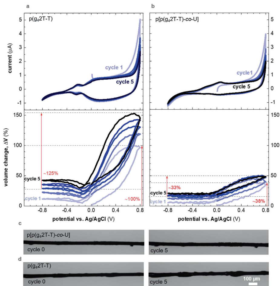
Figure 4. Cyclic voltammograms (top) and volume change of the polymer coating \Delta V = (V_{pol} - V_{pol}^0)/V_{pol}^0 , where V_{pol} is the volume of the coating at different potentials and V_{pol}^0 is the initial volume of the coating (bottom), recorded during oxidation/reduction cycle 1–5 of a carbon filament coated with \sim 2 \mu m of a) p(g_42T-T) and b) p[p(g_42T-T)-co-U] in 0.01 M KCl electrolyte; c,d) optical micrographs of the coated carbon filaments prior to the first cycle and after cycle 5.
