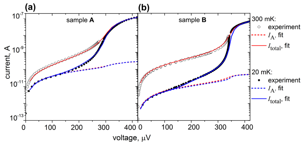
Figure 5. The fitting of IV-curves by HBE with Andreev current. (a) The sample A. (b) The sample B. The color legend from the right is valid for both (a,b) blue color is for 20 mK, red color is for 300 mK, dots are an experiment, solid curves are the total fitted current, the dashed curve shows Andreev current.
