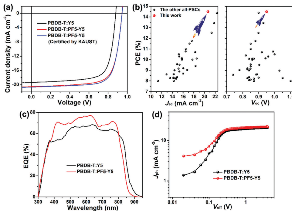
Fig. 2 (a) J - V plots of the PBDB-T:Y5-based PSCs and the PBDB-T:PF5-Y5-based all-PSCs under illumination with AM 1.5G, 100 mW cm -2 . (b) Plots of PCE against J_{sc} and PCE against V_{oc} for all-PSCs reported previously with PCEs over 8% and this study. (c) EQE plots of the PBDB-T:Y5-based PSCs and the PBDB-T:PF5-Y5-based all-PSCs, and (d) the corresponding photocurrent density ( J_{ph} ) versus effective voltage ( V_{eff} ) curves in this study.
