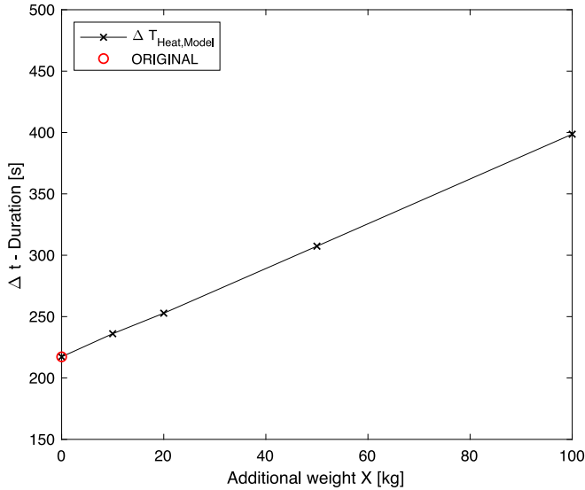
Fig. 15. Heating duration for the RDC plotted towards the relative increase of active thermal mass, modelled as an additional mass of the heat exchanger.
