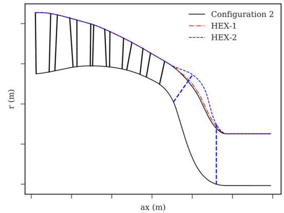
FIGURE 5: HUB AND SHROUD PROFILES OF THE INVESTIGATED HEX DUCT DESIGNS.
