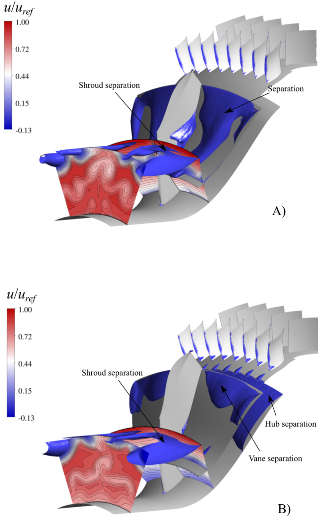
FIGURE 9: NORMALIZED AXIAL VELOCITY COMPUTED FOR THE HEX-1 (A) AND HEX-2 (B) DUCT DESIGN. THE ISO-SURFACE SHOWS REGIONS OF FLOW SEPARATION.
