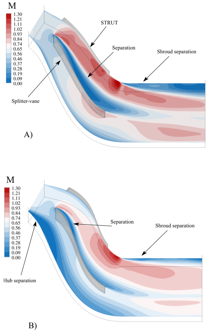
FIGURE 10: MACH NUMBER CONTOUR PLOT AT A CIRCUMFERENTIAL PLANE COMPUTED FOR HEX-1 (A) AND HEX-2 (B) DUCT DESIGN.
