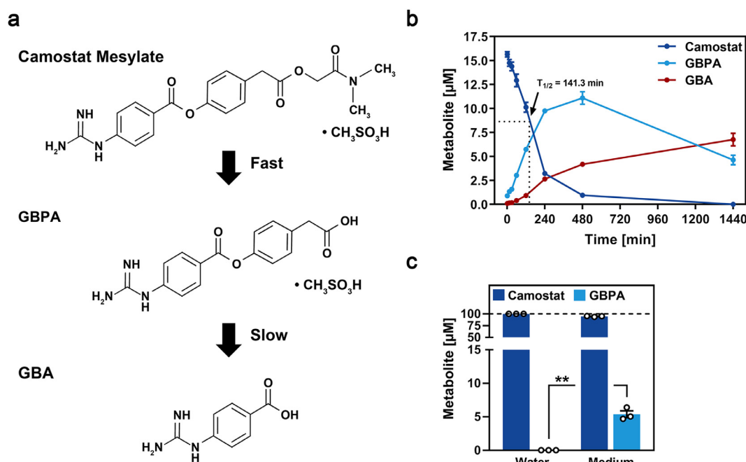
Fig. 6. Camostat mesylate is rapidly converted to GBPA in the presence of cell culture medium. (a) Metabolization of Camostat mesylate. (b) LC-MS/MS determination of Camostat, GBPA and GBA in culture medium containing FCS. Camostat mesylate was added to FCS-containing culture medium at a concentration of 15 μM. Samples were taken after incubation for 1, 15, 30, 60, 120, 240, 480, and 1,440 min at 37 °C, snap-frozen and stored at -80 °C. Samples were analyzed by LC-MS/MS and quantified regarding their content of intact Camostat mesylate and its metabolites GBPA (active) and GBA (inactive). Presented are the average (mean) data from three biological replicates (each performed with single samples). Error bars indicate the SEM. The turnover time that is required to cause metabolization of 50 % of Camostat mesylate (T 1/2 ) was further calculated by a non-linear regression model and was determined to be 141.3 min (95% confidence interval = 116.5 to 171.7 min). (c) Relative levels of Camostat mesylate and GBPA after incubation of 15 μM Camostat mesylate in either water or FCS-containing culture medium. For normalization, the combined values of Camostat mesylate and GBPA were set as 100% and the relative fractions of the compounds were calculated. Presented are the average (mean) data from three biological replicates (each performed with single samples). Error bars indicate SEM. Statistical significance of differences in GBPA levels following incubation of Camostat mesylate in either water or FCS-containing culture medium was analyzed by paired, two-tailed student's t-test (P = 0.0090). Abbreviations: FOY-51/GBPA = 4-(4-guanidinobenzoyloxy)phenylacetic acid; GBA = 4-guanidinobenzoic acid.
