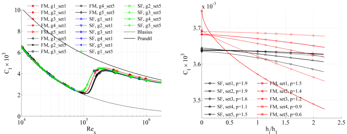
Figure 3 Influence of first cell size (set1 and set5) on the skin friction coefficient along the flat plate and convergence of friction coefficient C_F for SHIPFLOW and FINE TM /MARINE at \log_{10}(Rn) = 6.25
