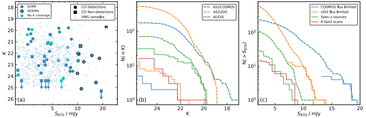
Figure 2. (a) K -band magnitude versus 870- \mu m flux density for sources targeted in this work (filled), with the parent samples of SMGs from AS2COSMOS, AS2UDS, and ALESS represented by the small points. For our targets, symbol shapes differentiate CO detections from non-detections. ALMA or NOEMA observations are differentiated by the symbol outline. Our sample covers the range of K magnitudes (median K = 22.3 ; 16–84th percentile range 20.7–23.5) spanned by the SMG population, while we typically select sources that are bright at 870 \mu m (median S_{870} = 5.9 mJy; 16–84th percentile range 2.8–10.5 mJy). 3\sigma upper limits for K non-detections are plotted, and we show a representative error bar for the whole population in the top right corner. Four sources are undetected in the K -band and 14 have no K -band photometry. In the latter cases we estimate K from the typical K - 3.6 \mu m colour at the appropriate redshift, where IRAC 3.6 \mu m coverage is available (cyan points). Seven of our targets have no K or IRAC 3.6 \mu m coverage, and therefore do not appear in this panel. (b): Cumulative histogram of K -band magnitude for our targets compared with their parent samples. Non-detected sources are shown at the relevant 3\sigma flux limit of their respective survey, as for simplicity are the seven sources that are not covered in K or IRAC 3.6 \mu m. We see that the K - and S_{870} -selected sources mostly sample the K -faint end of the parent sample, whereas the ALESS spec-z sources are complete above K \sim 21 . (c): Cumulative histogram of S_{870} for our targets compared with their parent samples. The S_{870} -selected scan -mode sources are mostly complete above \sim 15 mJy and \sim 10 mJy in AS2COSMOS and AS2UDS, respectively, whereas the K -selected and spec-z sources cover the fainter end of this parameter space.
