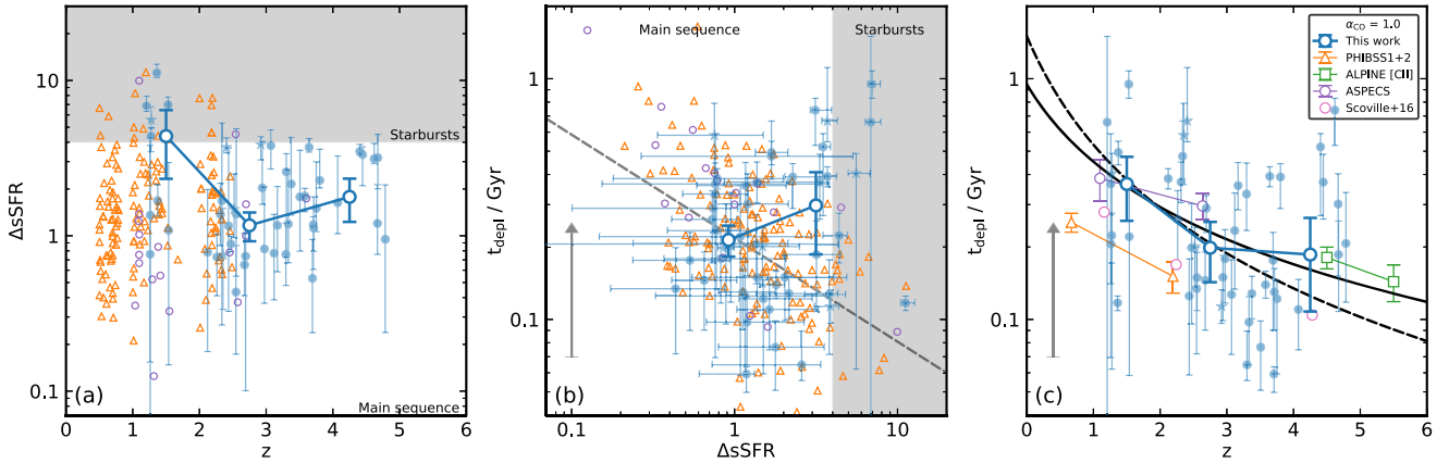
Figure 9. (a) Offset from the ‘main sequence’, \Delta\text{sSFR} = \text{sSFR}/\text{sSFR}_{\text{MS}} , versus redshift for our sample, using the Speagle et al. (2014) prescription for \text{sSFR}_{\text{MS}} . We indicate the region where \Delta\text{sSFR} > 4 , i.e. the loose definition of a ‘starburst’ galaxy. The majority of the SMGs lie below this region, with the binned averages (shown by the connected large open symbols in each panel) suggesting that at z = 2\text{--}5 the majority of our sample comprise apparently ‘main-sequence’ systems. (b) The variation of gas depletion timescale ( t_{\text{dep}} = M_{\text{gas}}/\text{SFR} ) with \Delta\text{sSFR} . We see no significant correlation between these two properties, although we caution that the two estimates are coupled as both use SFR. The dashed line shows the t_{\text{dep}} \propto \Delta\text{sSFR}^{-0.43} behaviour predicted by Tacconi et al. (2018) for CO-detected star-forming galaxies, which diverges from the trend for the SMG binned averages. (c) Gas depletion timescale, t_{\text{dep}} , versus redshift for our SMG sample. We also plot the PHIBSS CO-detected galaxies, a compilation of star-forming galaxies from Scoville et al. (2016), and [C II]-detected galaxies from the ALPINE survey (Dessauges-Zavadsky et al. 2020). Our SMGs have a median t_{\text{dep}} = 210 \pm 40 Myr and the binned averages show a moderate decline across z \sim 1\text{--}5 . The dashed line shows the prediction of Davé, Finlator & Oppenheimer (2012) – t_{\text{dep}} \propto (1+z)^{-1.5} , and the solid line shows our own fit of the form t_{\text{dep}} \propto (1+z)^a to our binned data, from which we estimate a = -1.1 \pm 0.3 at fixed stellar mass and \Delta\text{sSFR} . In (b) and (c), we show a vector indicating by how much points would move if we were to adopt \alpha_{\text{CO}} = 3.6 instead of \alpha_{\text{CO}} = 1 .
