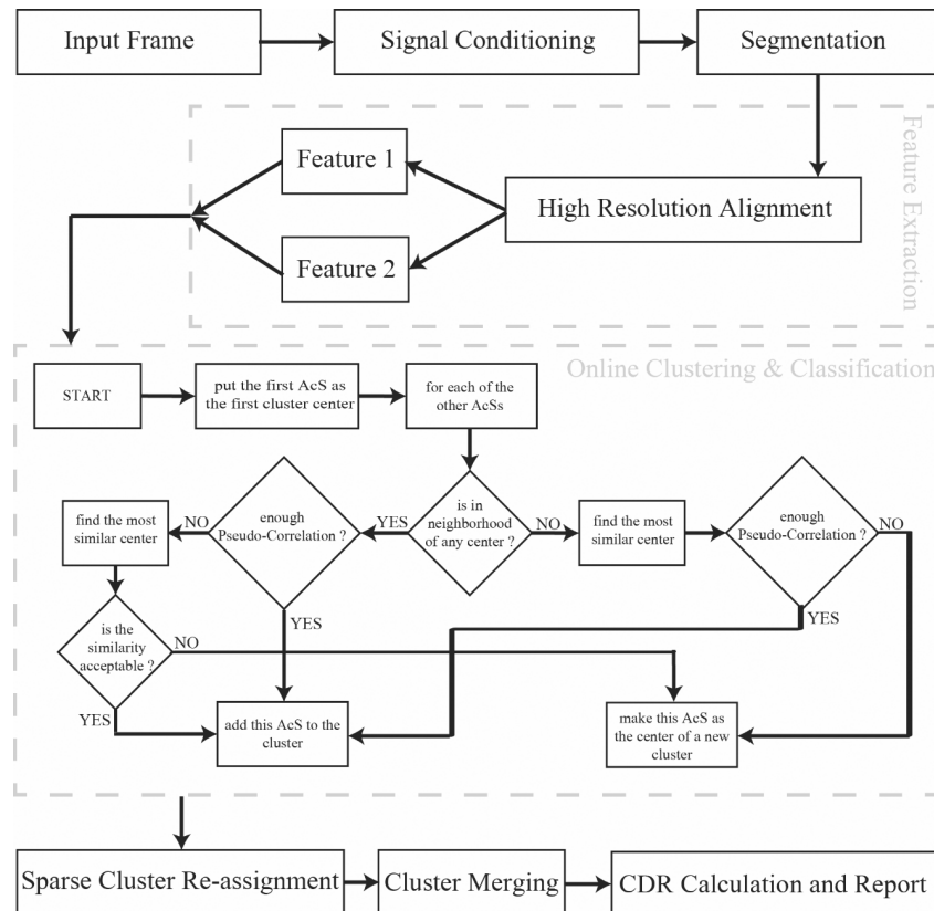
Fig. 1. The main flowchart of the proposed online intra-muscular EMG signal decomposition algorithm. AcS: active segment; CDR: cumulative discharge rate.
