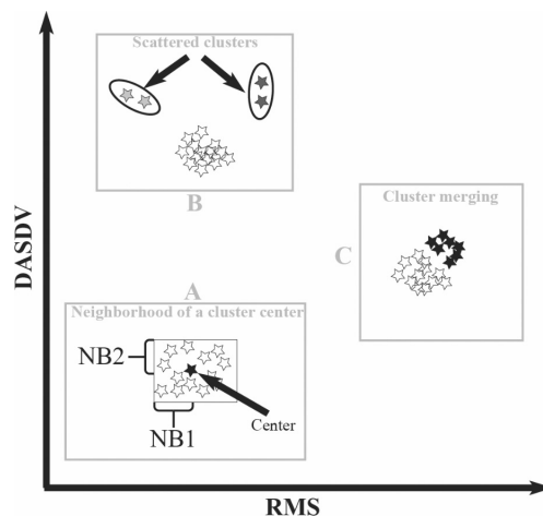
Fig. 2. The definition of neighborhood of a cluster center.
