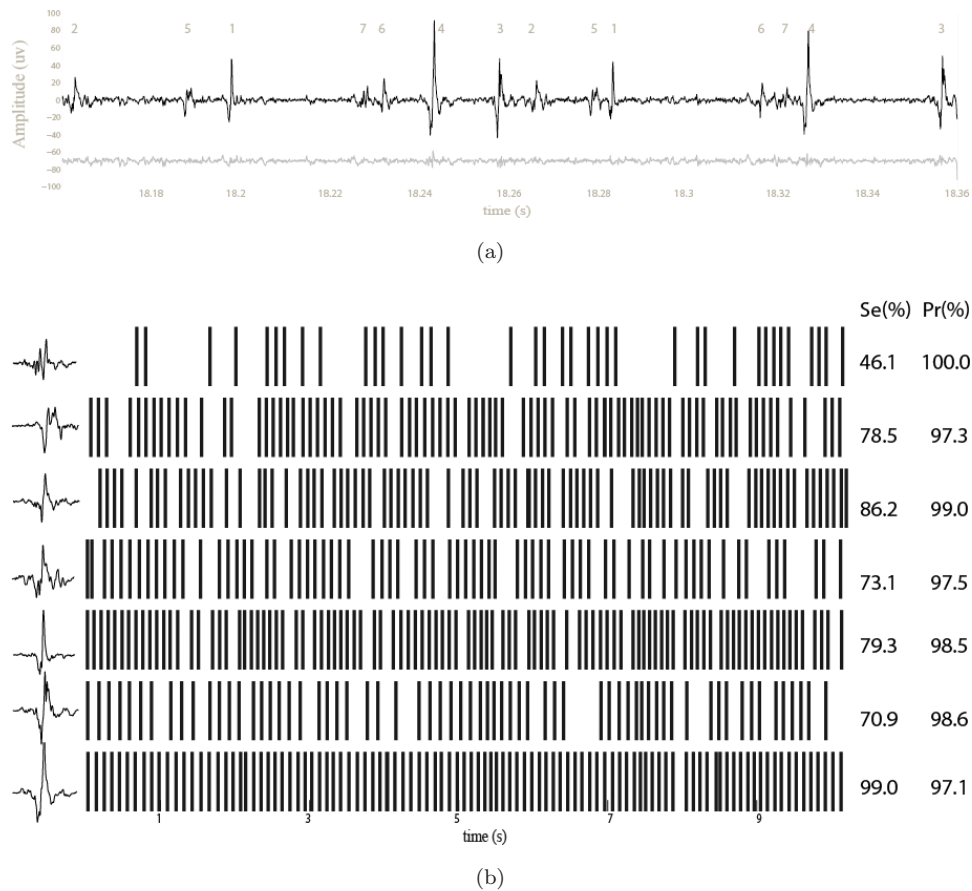
Fig. 3. (A) The result of decomposing a 10 s iEMG signal from BFlh at 5% MVC. None of the MUs were missed and No erroneous MUs were detected by the proposed algorithm. A segment of the EMG signal (high-pass filtered at 1 kHz, top trace) and the residual signal after decomposition (bottom trace). The numbers at the top indicate the identified MU discharges. (B) The templates of the identified MUs (left), the identified discharge times of each MU (middle), and the identification sensitivity and precision of each MU (right). The overall sensitivity (Se), precision (Pr) and accuracy of the algorithm were 76 \pm 16 , 98 \pm 1 , and 75 \pm 16 , respectively.
