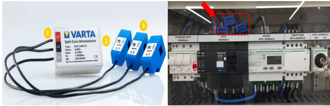
Fig. 6. Split-core current sensor.
