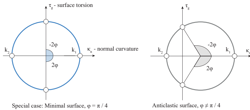
Figure 3: Mohr's circle of curvature where the axis represents the normal curvature \kappa_n and surface torsion \tau_g . The blue circle represent a minimal surface where \kappa_1 and \kappa_2 are of equal magnitude with opposite sign, therefore the asymptotic directions are given with \phi = \pi/4 and form right angles. For the grey case \phi \neq \pi/4 and therefore the asymptotic directions are not orthogonal to each other.
