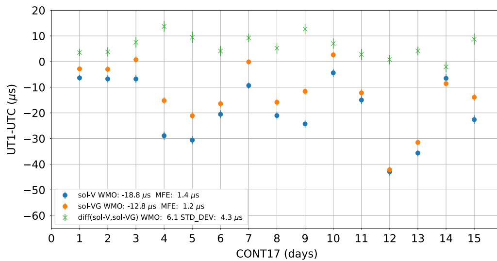
Fig. 11 UT1 estimates and differences between sol-V and sol-VG. Presented are weighted mean offset (WMO) and mean formal error (MFE)
