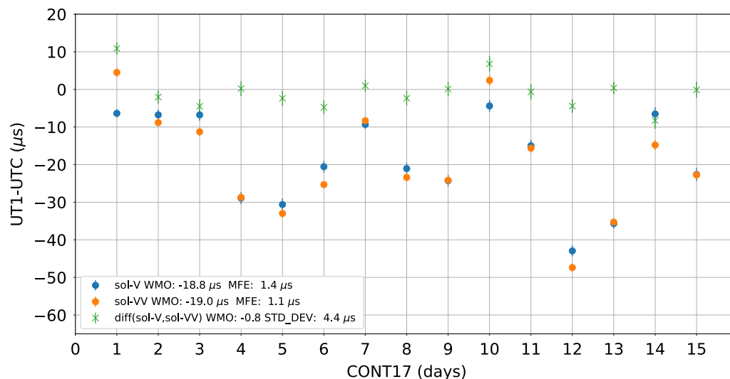
Fig. 12 UT1 estimates and differences between sol-V and sol-VV. Presented are weighted mean offset (WMO) and mean formal error (MFE)
