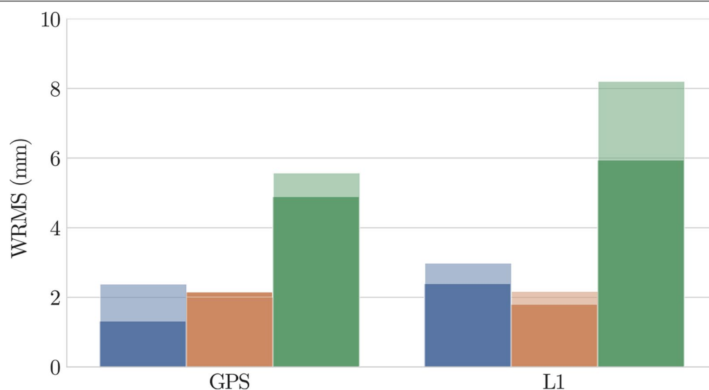
Fig. 5 Average station position repeatabilities (WRMS in mm) for the two co-located networks (VLBI L1 sites on the right and GPS sites on the left) for a single-technique solutions, i.e., sol-V and sol-G, (faded) and b the combined solution sol-VG (colored). The results are computed based on the 15 daily solutions. The components evaluated are north (blue), east (orange) and up (green) of the local topocentric frame
