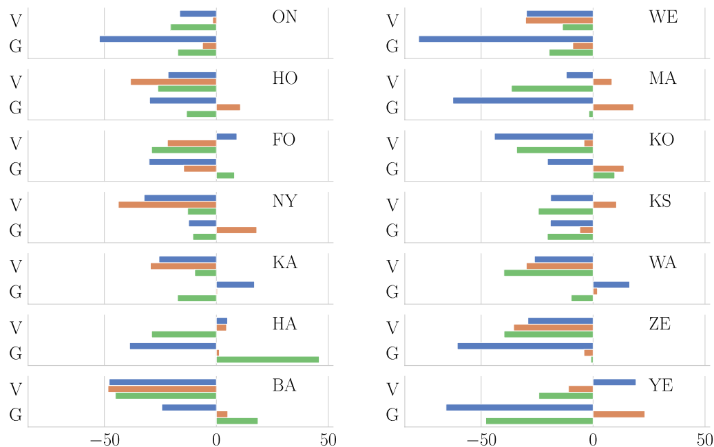
Fig. 8 Relative change in repeatabilities (%) per station for the two co-located networks between between sol-V and sol-VG as well as sol-G and sol-VG. Negative repeatability changes mean that the combined solution lowers the repeatability, i.e., improvement. The components evaluated are north (blue), east (orange) and up (green) of the local topocentric frame
