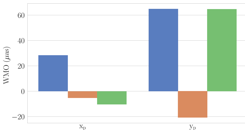
Fig. 14 Polar motion ( x_p, y_p ) weighted mean offsets (WMO) w.r.t. IGS PM products for sol-V (blue), sol-VG (orange), and sol-VV (green)
