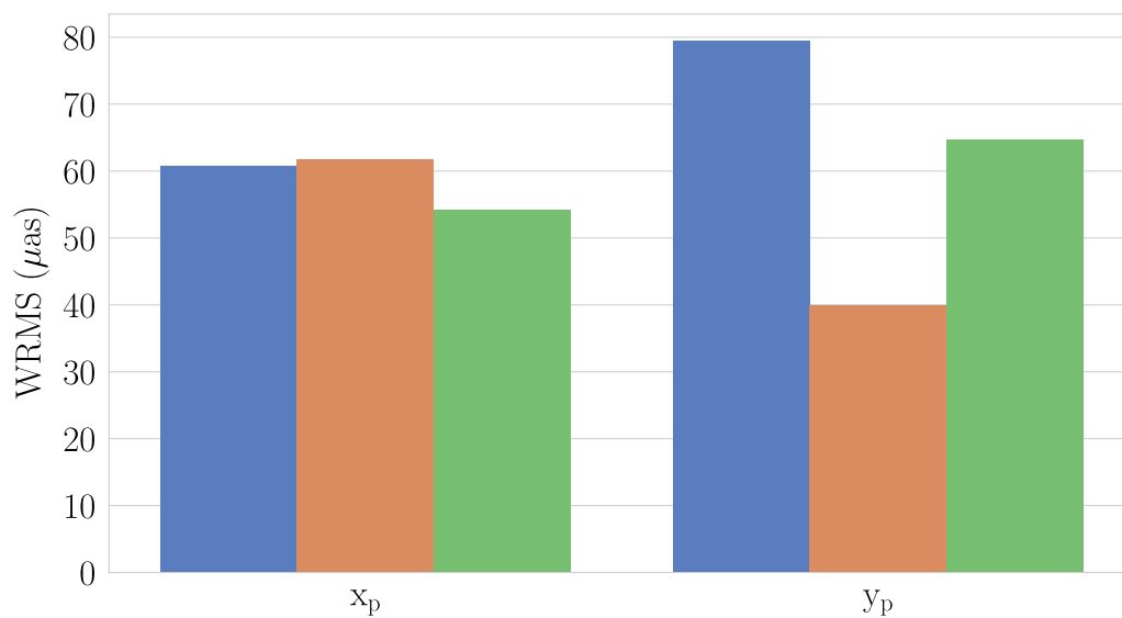
Fig. 13 Polar motion ( x_p, y_p ) WRMS differences w.r.t. IGS PM products for sol-V (blue), sol-VG (orange), and sol-VV (green)
