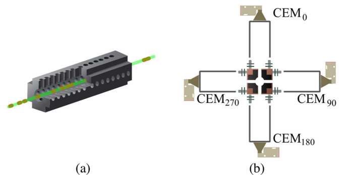
FIG. 3. (a) shows one of the two graphite tubes inside PEARLS within which the ion and photon beams interact. The photoelectrons escape through the small holes on the sides of the tube or are absorbed by the graphite surfaces. (b) Cross section of one detector plane of PEARLS used in the current experiment.
