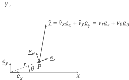
Figure 4: A point P with Cartesian coordinates (x, y) and cylindrical coordinates (r, \theta) , where x = r \cos \theta and y = r \sin \theta . A vector \check{v} , with tail in P , with Cartesian components (\check{v}_x, \check{v}_y)^T and cylindrical components (v_r, v_\theta)^T .
