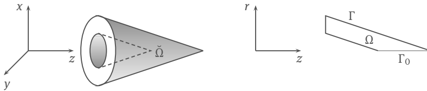
Figure 3: A right circular cone with a hole. Each corner of \Omega contained in the z -axis corresponds to a conical singularity in \partial\check{\Omega} , except if the opening angle of \Omega at this point is \pi/2 . Each remaining corner of \Omega generates an edge in \partial\check{\Omega} .
