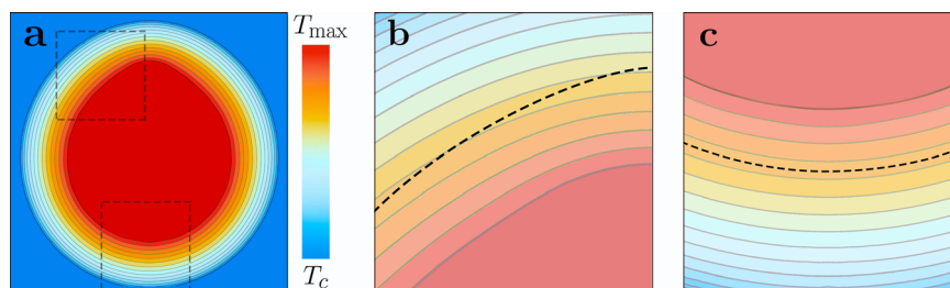
Fig. 4 Isotherms around a non-spherical particle. a Composition profile \phi(r) in the vicinity of an axisymmetric particle with a surface temperature above the critical value T_c of water-2,6-lutidine. \phi is constant at the isothermal surface and decreases with distance; the dark blue area indicates the range where T \leq T_c and where the composition takes the bulk value \phi_c . The gray lines in the critical droplet ( T \geq T_c ) indicate iso-composition surfaces. b The curvature of the top of the particle is larger than that of its bottom; as a consequence, \phi varies more rapidly close to the top and the iso-composition lines are denser. The dashed line, at a constant distance from the particle surface, crosses iso-composition lines; thus there is a composition gradient \nabla_\parallel \phi parallel to the surface, which induces a diffusio-osmotic creep velocity and results in self-propulsion of the particle. Our detailed analysis relates the particle velocity to the Fourier series of the particle shape R(\theta) . c Instead, the bottom of the particle is almost spherical with roughly constant curvature and zero creep velocity.
