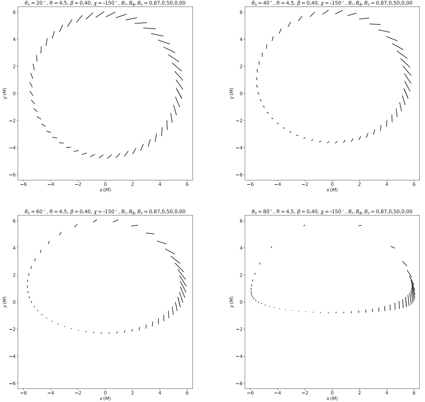
Figure 6. Polarization patterns for four models with equatorial magnetic field and emission radius R = 4.5 , viewed at different inclination angles. Top left: \theta_o = 20^\circ . Top right: \theta_o = 40^\circ . Bottom left: \theta_o = 60^\circ . Bottom right: \theta_o = 80^\circ . All the models have velocity angle \chi = -150^\circ , and magnetic field trailing opposite to the velocity ( \eta = \chi + 180^\circ ). The model in the top left, rotated counter-clockwise by 288^\circ and with emission spread over a finite range of radii, is shown in Figure 9 as a toy model of M87*.
