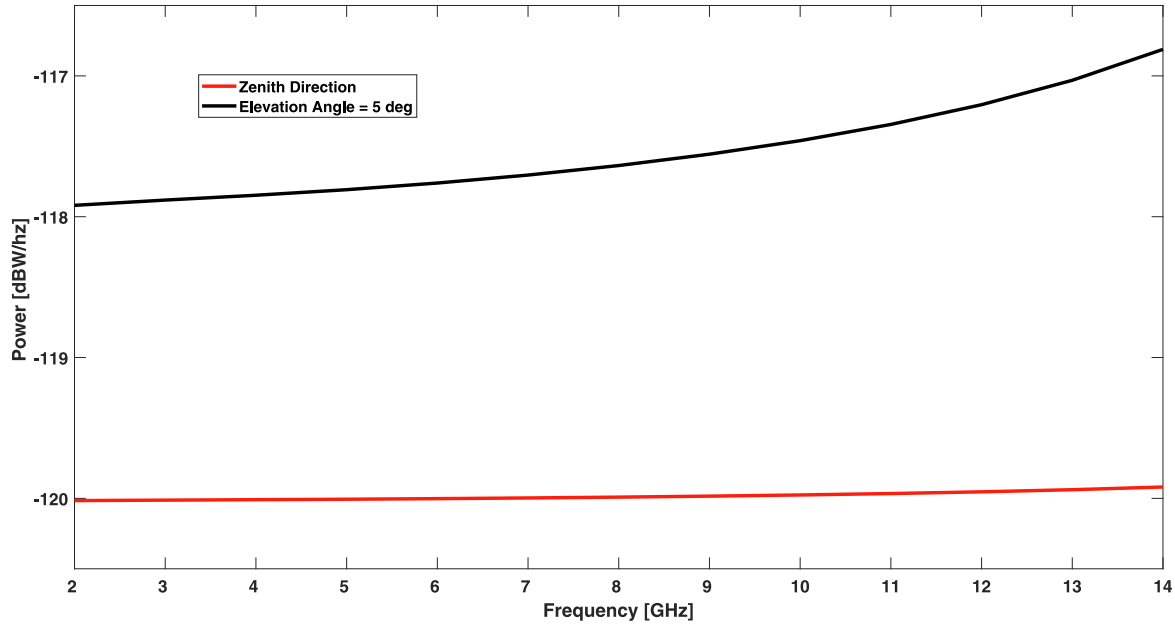
Fig. 5. Required transmitted power in the zenith direction (red line) and at \epsilon = 5^\circ (black line) over the frequency range 2–14 GHz from the total link budget. The elevation dependent increase in loss is more pronounced than that of the frequency dependency especially at the higher frequencies resulting from the atmospheric attenuation.
