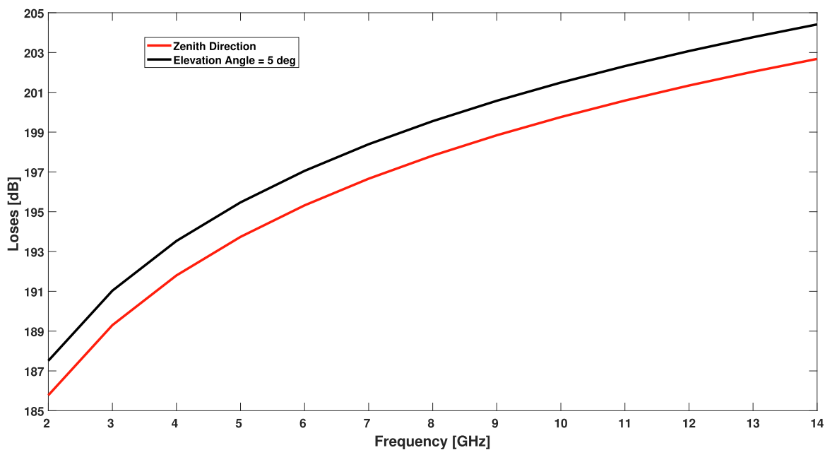
Fig. 3. Free-space path loss in the zenith direction (red line) and at \epsilon = 5^\circ (black line) over the frequency range 2–14 GHz. The difference in FSPL at the highest and lowest frequency is about 17 dB. The elevation dependent effect is much smaller than the frequency dependent increase.
