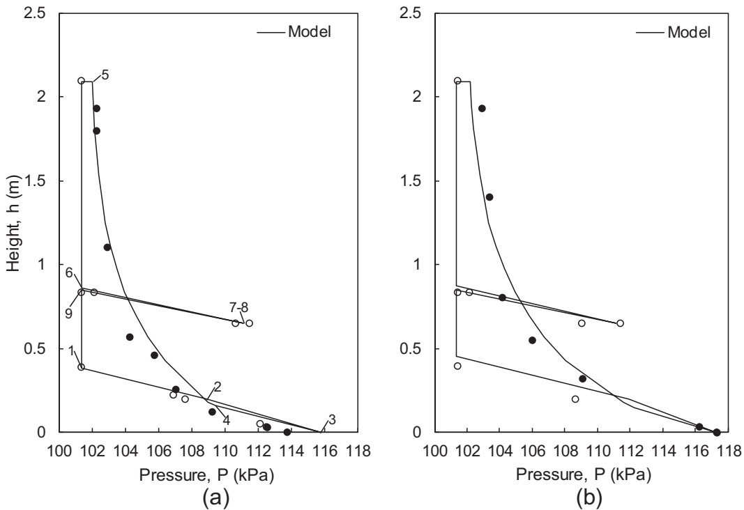
Fig. 5. Pressure loops obtained by the model compared with measurements from the CFM at TU-Wien: (a) W_t = 105 kg, Q_t = 353.5 \text{Nm}^3/\text{h} , Q_2/Q_t = 0.18 , Q_{bb}/Q_t = 0.06 ; (b) W_t = 130 kg, Q_t = 396.8 \text{Nm}^3/\text{h} , Q_2/Q_t = 0.5 , Q_{bb}/Q_t = 0.15 (solid circles represent measurements from the riser, while open circles those from the rest of the system; the point at height 0 m was not measured but estimated with the porosity given by the model for the dense zone of each test; in (a), numbers represent the pressures given by the model for points shown in Fig. 1a).
