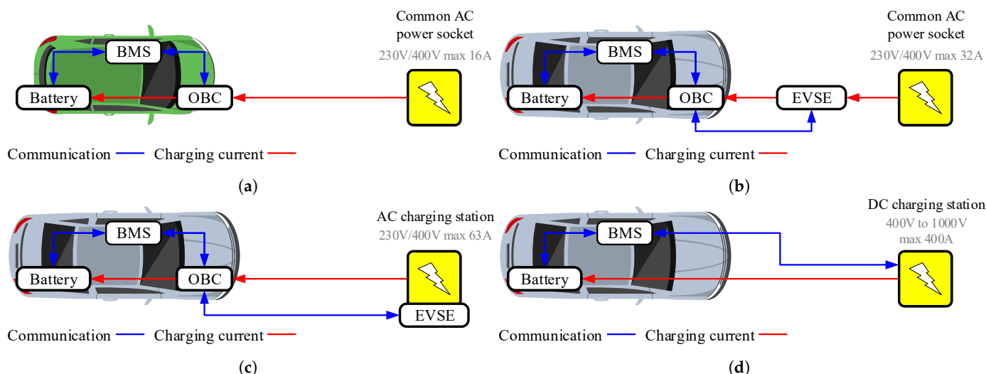
Figure 1. Illustration of the four charging modes as described in [12]. (a) Charging mode 1. (b) Charging mode 2. (c) Charging mode 3. (d) Charging mode 4.
