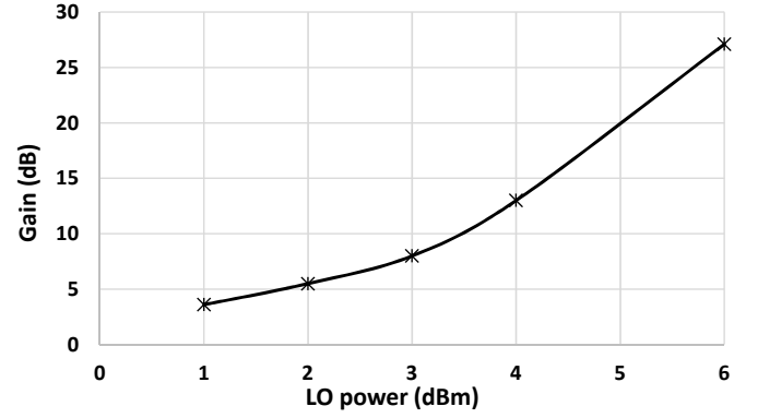
Fig. 12. Receiver measured gain versus LO input power at 130 GHz and 1 GHz IF.
