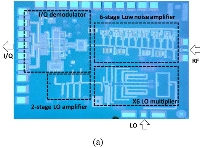
Fig. 5. (a) The fabricated chip photo of direct conversion I/Q receiver. The chip area is 1.4 \times 1.1 mm 2 . (b) Simplified block diagram of measurement setup for characterization of the transmitter MMIC chip.
