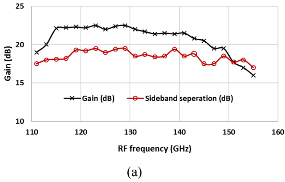
Fig. 6. (a) Transmitter measured upper sideband gain and sideband suppression versus RF frequency. (b) Transmitter measured gain versus IF frequency at fixed 22 GHz LO.
