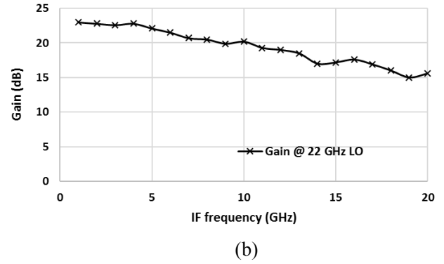
Fig. 6. (a) Transmitter measured upper sideband gain and sideband suppression versus RF frequency. (b) Transmitter measured gain versus IF frequency at fixed 22 GHz LO.
