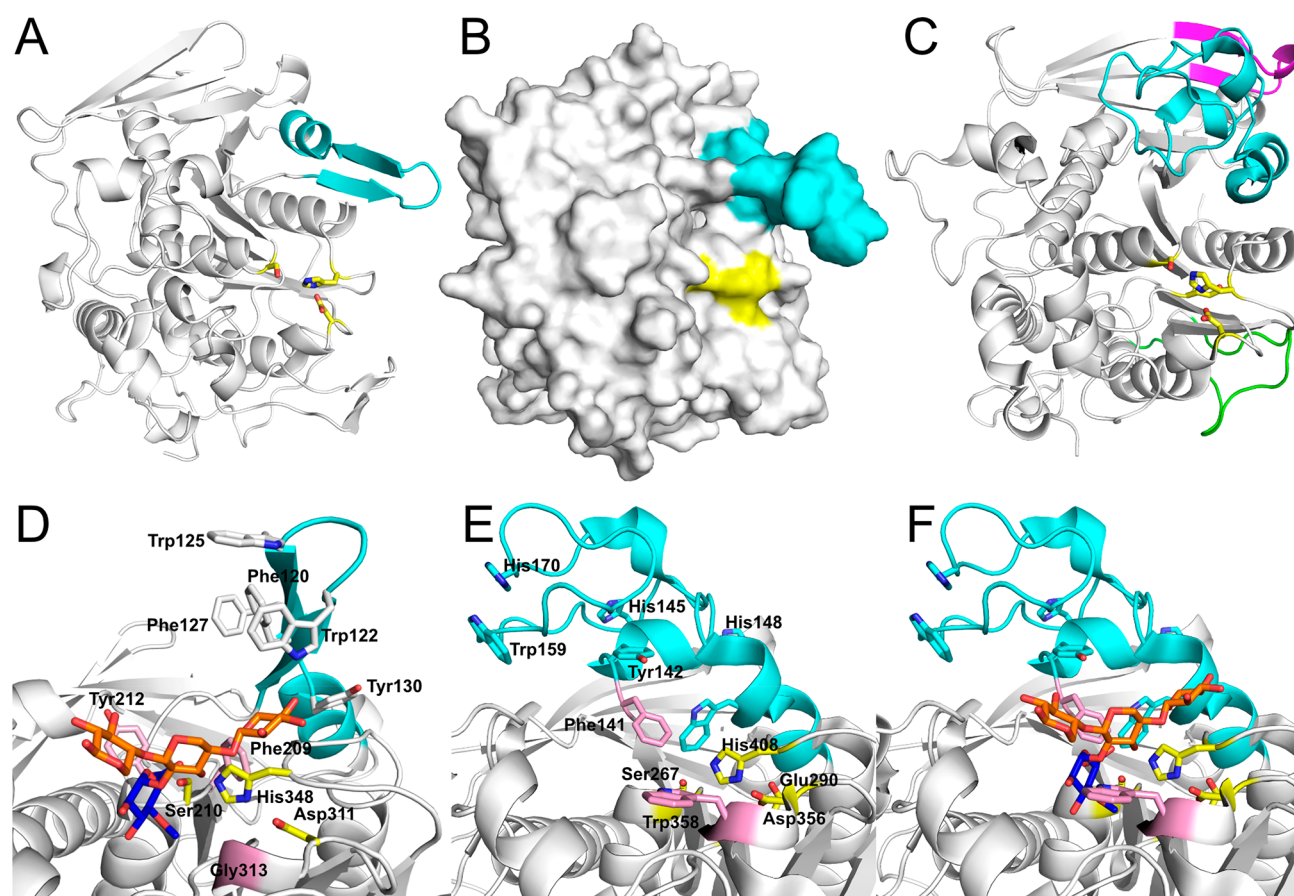
Figure 5. Overall fold and active site of CkGE15A and comparison to OtCE15A (PDB entry 6T0I 27 ). Catalytic residues are shown as yellow sticks, and Reg2 is colored cyan. (A) Overall fold of CkGE15A . (B) Surface view of CkGE15A . (C) Overall fold of OtCE15A , with Reg1 colored magenta and Reg3 colored green. (D) Close-up of the CkGE15A active site, with catalytic residues shown as yellow sticks, aromatic residues in Reg2 shown as white sticks, and other potentially important binding residues colored pink. The tetrasaccharide 2 3 -(4- O -methyl- \alpha -D-glucuronyl)-xylotriase (XUX) from the OtCE15A crystal structure is superimposed and shown as sticks with xylose moieties colored orange and GlcA colored blue. (E) Close-up of the OtCE15A active site with catalytic residues shown as yellow sticks and aromatic residues involved in substrate binding shown as pink sticks. (F) Close-up of the OtCE15A active site with the bound XUX molecule shown as sticks with xylose moieties colored orange and GlcA colored blue.
