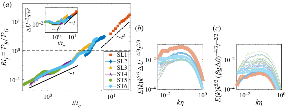
Figure 2. Temporal scalings of the turbulent kinetic energy: (a) ratio between the buoyancy and gradient the production (i.e. the flux Richardson number R_{if} ) integrated over the wall-normal direction, with the inset showing the scaling of \overline{u'w'} at the centreline; energy spectra normalised with the (b) shear and (c) RT scalings for all the simulations (see (4.4)); the line thickness is proportional to the non-dimensional time.
