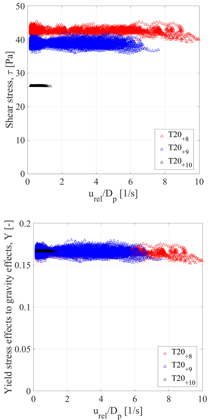
Fig. 8. a) Shear stress, \tau , vs. shear rate, \frac{u_{rel}}{D_p} of the rising tracers. b) Yield stress effects to gravity effects, Y vs. shear rate, \frac{u_{rel}}{D_p} of the rising tracers.
