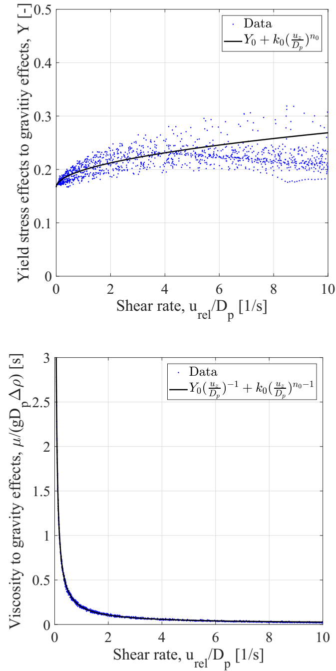
Fig. 7. Fitting of a) the Yield stress effects to gravity effects, Y and b) the viscosity to gravity effects vs. shear rate, \frac{u_{rel}}{D_p} .
