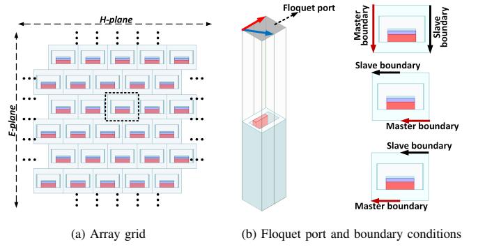
Fig. 2. Infinite array model
