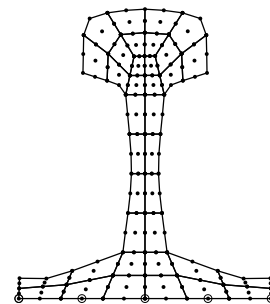
Figure 3: The discretized cross-section of the rail. Encircled nodes on the rail foot are used to couple the WFE model to the receptance of the support.
