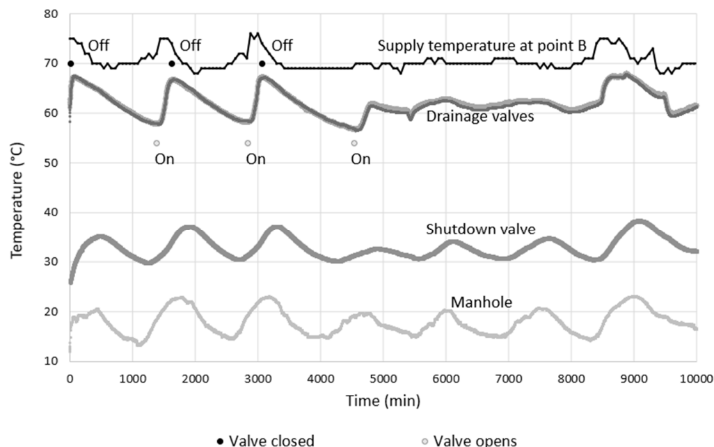
Figure 11. Temperature measurements during the three shutdowns (i.e., off to on) followed by normal operation starting at approximately 4500 min.
