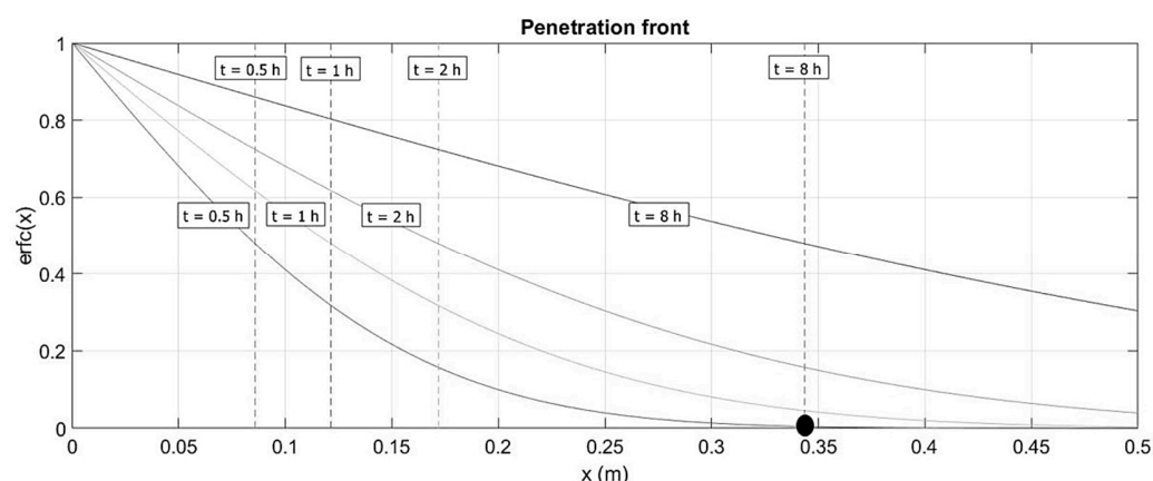
Figure 7. Progress of the heat front in a stainless-steel rod for times ranging from 0.5 to 8 h; dashed lines represent how deep into the material half of the possible temperature change has progressed.
