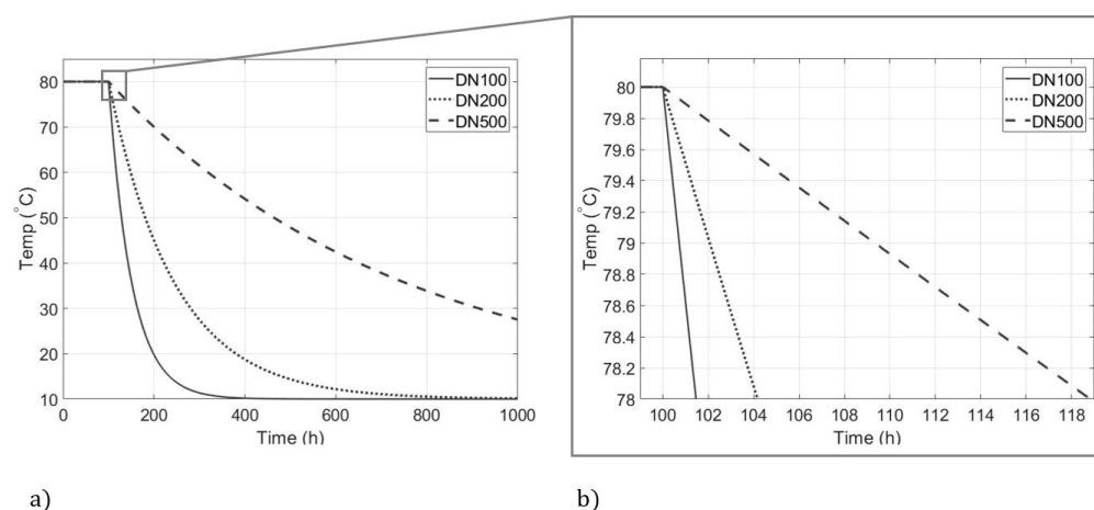
Figure 3. (a) Expected cooling times for pipes of different dimensions; (b) close-up of expected temperature declines during a shutdown; MATLAB model according to Section 2.1.1, T_s fixed at 10 °C.
