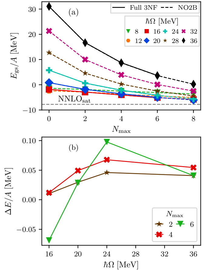
FIG. 6. (a) The ground-state energy per particle of ^{16}\text{O} computed with the N2LO sat interaction for different \hbar\Omega . The solid lines show results with full inclusion of the 3NF (only available for a subset of HO frequencies and up to N_{\max} = 6 ), while the dashed lines correspond to NO2B-approximated 3NF. The horizontal dashed line is the converged N2LO sat result computed with the CC method [32]. (b) The NO2B-approximation error \Delta E \equiv E_{\text{gs}}^{3\text{NF}} - E_{\text{gs}}^{\text{NO2B}} per particle where E_{\text{gs}}^{3\text{NF}} and E_{\text{gs}}^{\text{NO2B}} are the ground-state eigenenergies of Eqs. (1) and (20), respectively.
