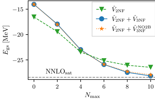
FIG. 3. The ground-state energy of ^4\text{He} computed with the N2LO sat interaction for fixed basis frequency \hbar\Omega = 20 MeV. The result with only the 2NF interaction (green, dashed line) is compared with the full Hamiltonian including 3NFs (blue, solid line) and with the NO2B-approximated one (orange, dotted line), corresponding to Eqs. (1) and (20), respectively. The dashed horizontal line indicates the converged N2LO sat ground-state energy E_{\text{gs}} = -28.43 MeV [32].
