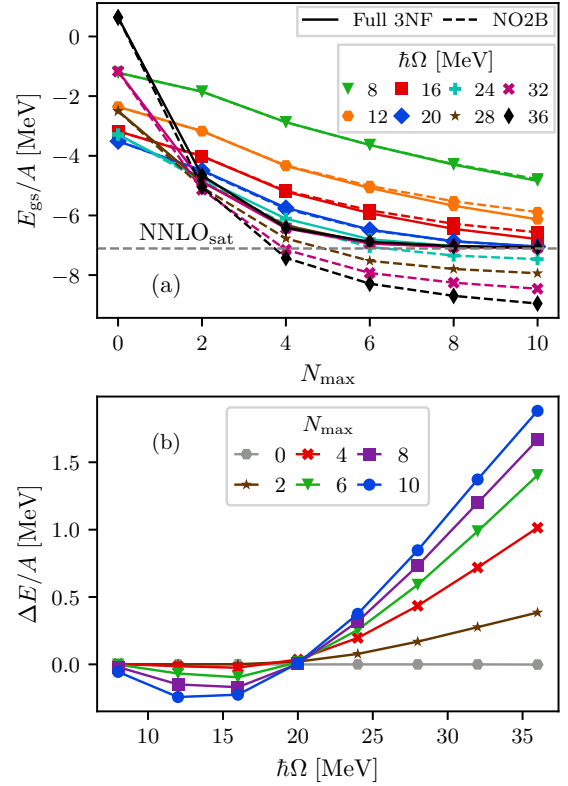
FIG. 4. (a) The ground-state energy per nucleon of ^4\text{He} computed with the N2LO sat interaction for different \hbar\Omega . The solid lines show results with full inclusion of the 3NF, while the dashed lines correspond to NO2B-approximated 3NF. Although the convergence rate is \hbar\Omega dependent, the full 3NF results converge towards the exact result (horizontal dashed line) while the results with the NO2B approximation do not. (b) The NO2B-approximation error \Delta E \equiv E_{\text{gs}}^{3\text{NF}} - E_{\text{gs}}^{\text{NO2B}} per nucleon where E_{\text{gs}}^{3\text{NF}} and E_{\text{gs}}^{\text{NO2B}} are the ground-state eigenenergies of Eqs. (1) and (20), respectively.
