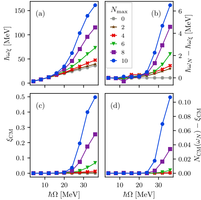
FIG. 5. CM analysis for ^4\text{He} eigenstates obtained with the NO2B Hamiltonian. The frequency \hbar\omega_\xi from Eq. (27) is shown in panel (a) and the difference \hbar\omega_N - \hbar\omega_\xi is shown in panel (b). Note that the basis frequency \hbar\Omega is equal to both \hbar\omega_N and \hbar\omega_\xi at N_{\max} = 0 , as shown by the gray line with circle markers. The CM metric \xi_{\text{CM}} from Eq. (41) is shown in panel (c) and the difference N_{\text{CM}}(\omega_N) - \xi_{\text{CM}} in panel (d).
