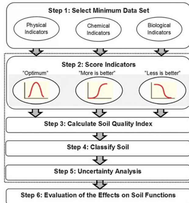
Figure 3-6. A generic framework for soil function assessment. The dotted box corresponds to operations carried out in the SF Box tool, from (Volchko et al., 2014a).
