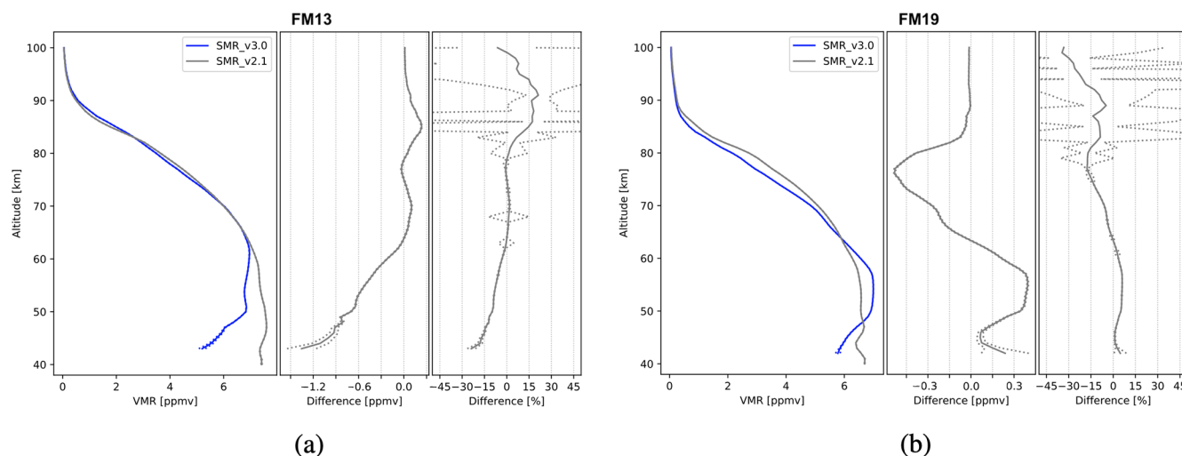
Figure 6. Comparison of SMR v3.0 with respect to v2.1 \text{H}_2\text{O} profiles, from FM13 (a) and FM19 (b). The data plotted are global averages over the time period between February 2001 and April 2019. Each subfigure consists of three panels. Left panels show volume mixing ratios, expressed in ppmv. Centre panels show absolute differences, expressed in ppmv. Right panels show relative differences, expressed in percentage. The differences shown are calculated as medians of the single profiles' differences. The dashed lines represent the standard deviation of the median which, in some cases, is smaller than the thickness of the profile line, causing the dashed line not to be distinguishable.
