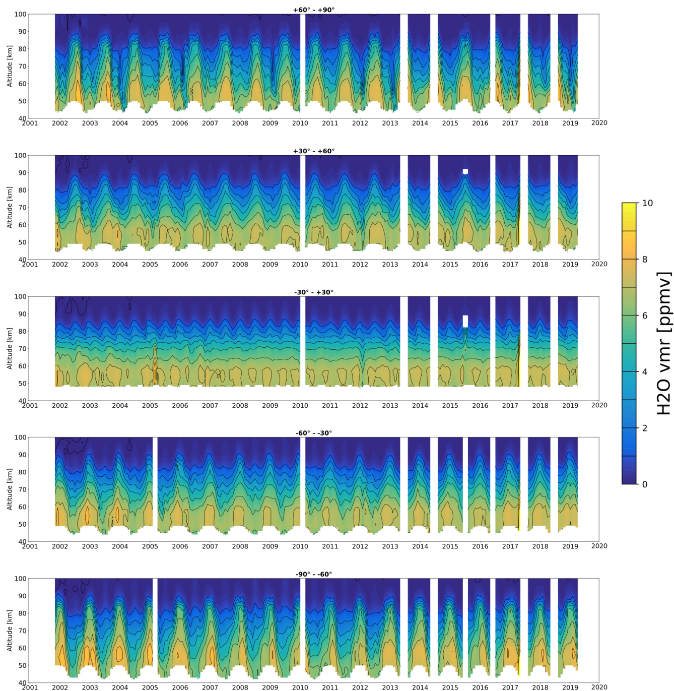
Figure 4. Time series of FM19 \text{H}_2\text{O} volume mixing ratios measured by SMR for different latitude bands. The white areas indicate periods and altitudes at which the number of measurements in the given latitude band is lower than 10. The ticks on the x axis correspond to the beginning of each year.
