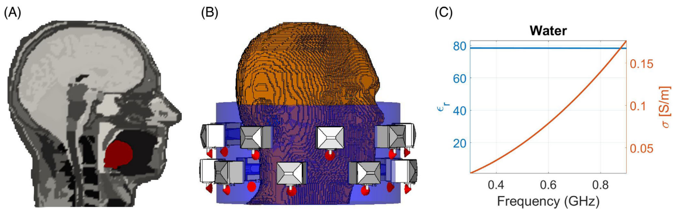
FIGURE 3 (A) Cross-section of the patient model with a large tumor shown in red in the tongue region. (B) CST model of the patient along with a 16-element elliptical array of open ridged-waveguide (ORWG) antennas and (C) the dielectric properties of the first-order Debye model of water used in the simulation [Color figure can be viewed at wileyonlinelibrary.com]
