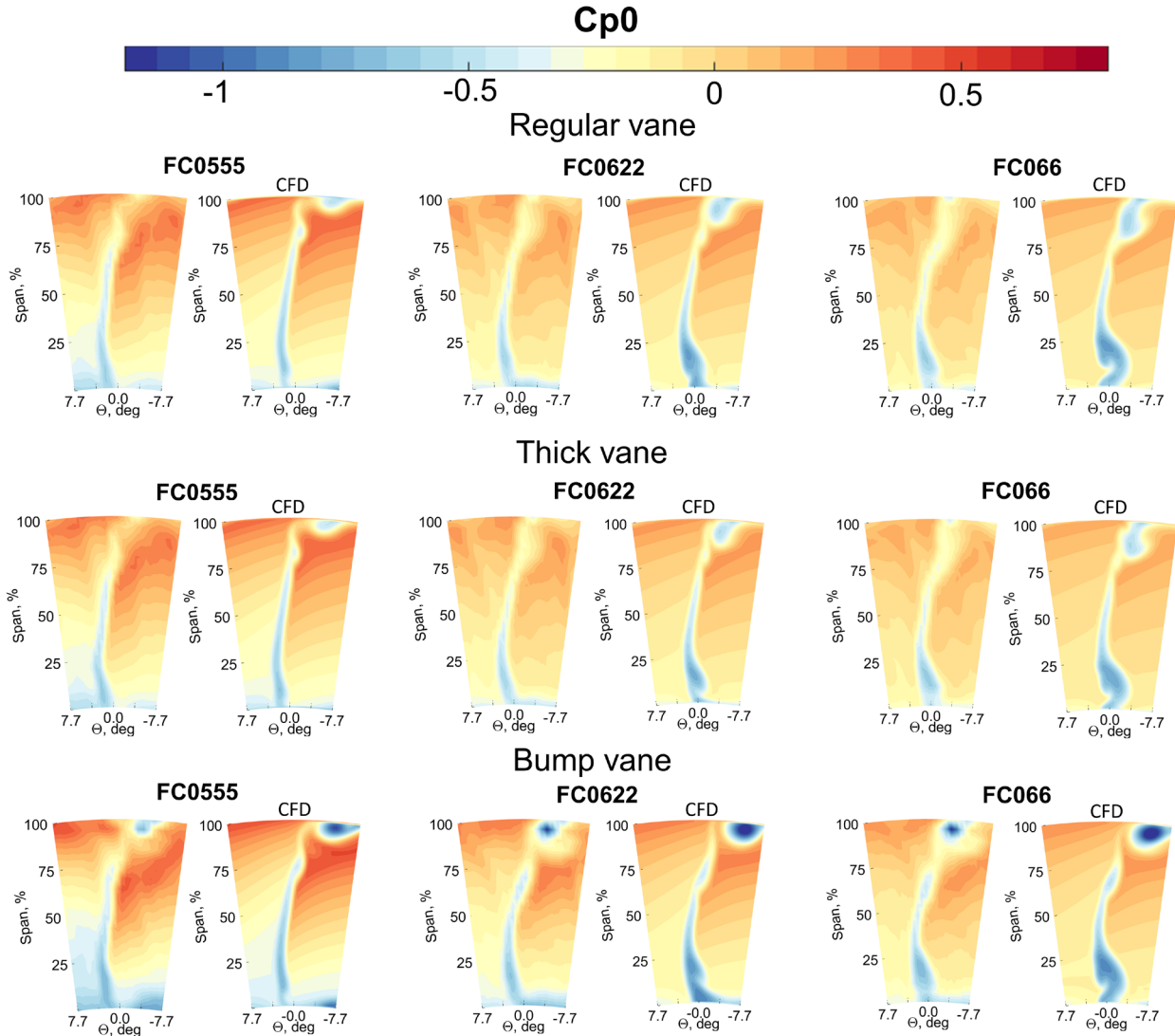
FIGURE 12: Total pressure coefficient distributions at Outlet plane for regular, thick, and bump vanes at on- and off-design flow coefficients. In each contour plot: PS – to the left, SS – to the right.
