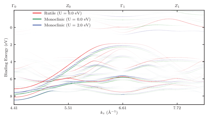
FIG. 8. Band structure plot similar to Fig. 7, but along the \Gamma - Z direction at k_x = -1.37 \text{ \AA}^{-1} for the nonmagnetic rutile phase for U = 0.0 eV [red, Fig. 4(b)] and the antiferromagnetic monoclinic phase for U = 0.0 eV (green) and 2.0 eV [blue, Fig. 4(e)].
