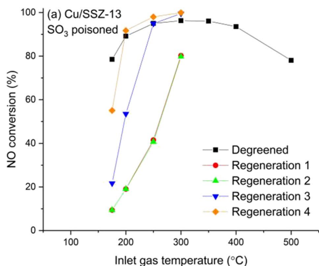
Fig. 10 Fast SCR activity (NO conversion) of degreened catalysts and during regeneration of \text{SO}_3 -poisoned a Cu/SSZ-13 and b Cu/BEA. Feed: 200 ppm NO, 200 ppm \text{NO}_2 , 400 ppm \text{NH}_3 , 8% \text{O}_2 , 5%
