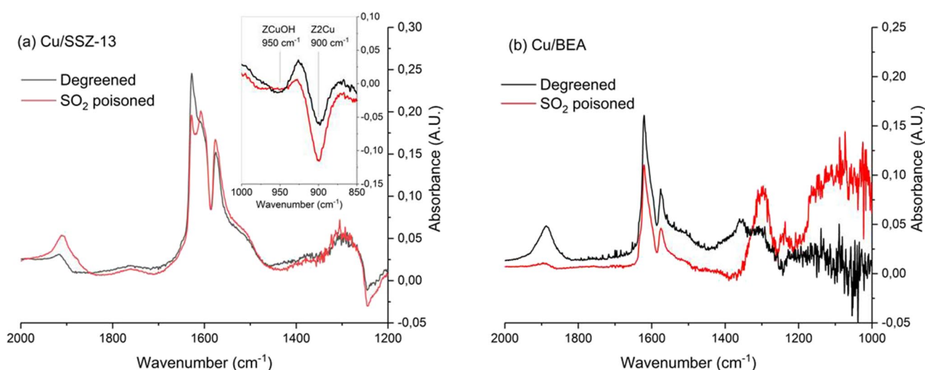
Fig. 11 DRIFT spectroscopy absorbance spectra of NO at 30 °C after oxidizing pretreatment at 500 °C of degreened and \text{SO}_2 -poisoned a Cu/SSZ-13 and b Cu/BEA catalysts. The spectra were recorded after 55 min of NO exposure
