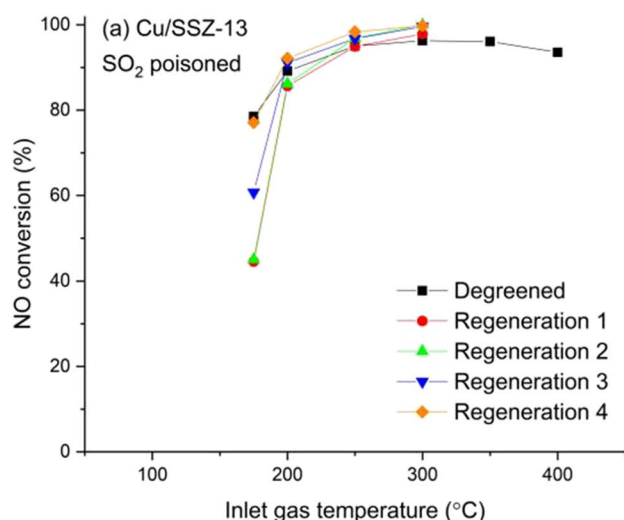
Fig. 9 Fast SCR activity (NO conversion) of degreened catalysts and during regeneration of \text{SO}_2 -poisoned a Cu/SSZ-13 and b Cu/BEA. Feed: 200 ppm NO, 200 ppm \text{NO}_2 , 400 ppm \text{NH}_3 , 8% \text{O}_2 , 5% \text{H}_2\text{O}
