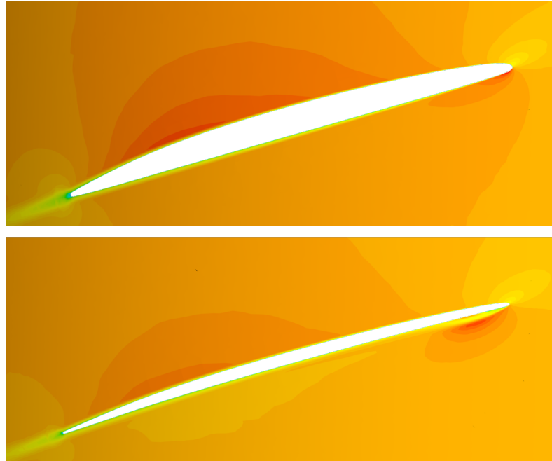
Figure 9: Ship-Scale CFD results; contours of velocity magnitude in a reference frame rotating with the propeller at a radial section at r/R = 0.9 . Ice classed propeller (top) and conventional propeller (bottom). Contour scale 0-23 m/s.
